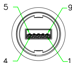
PIN ASSIGNMENT FRONT VIEW (前視圖)
