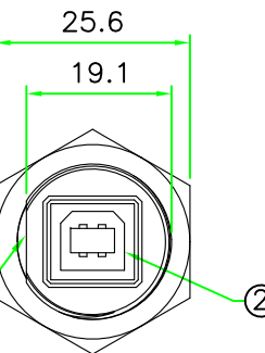
FRONT VIEW (前視圖)
