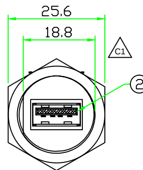
FRONT VIEW (前視圖)
