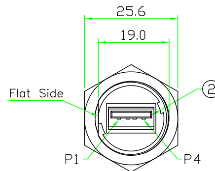
FRONT VIEW A1 (前視圖)
