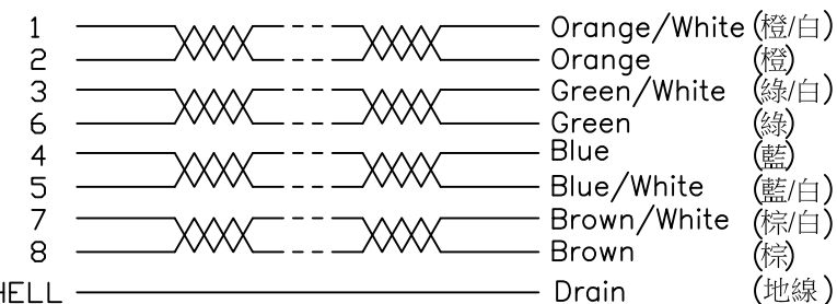
RJ45 PLUG
