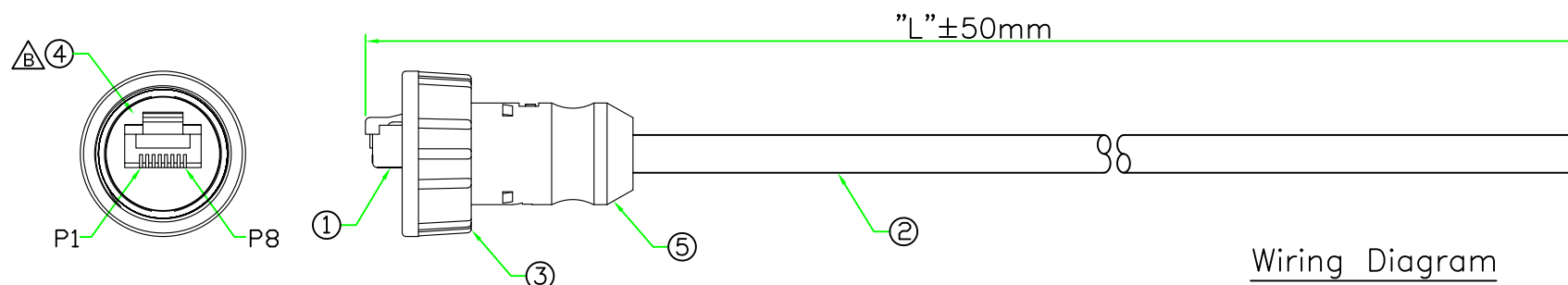
RJ45 PLUG
