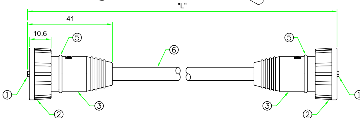
WIRING DIAGRAM △
