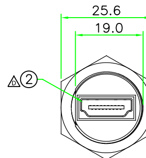
FRONT VIEW (前視圖)
