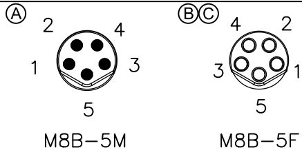
PIN ASSIGNMENT FRONT VIEW (前視圖)
