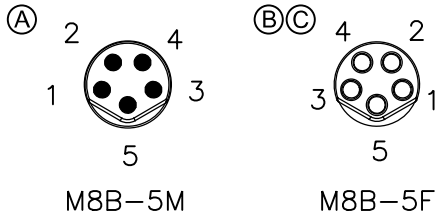
PIN ASSIGNMENT FRONT VIEW (前視圖)
