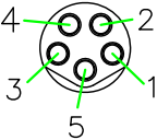
PIN ASSIGNMENT FRONT VIEW 正視圖
