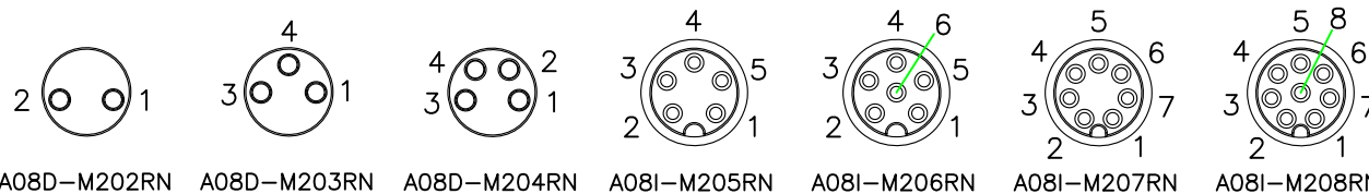
PIN ASSIGNMENT FRONT VIEW (前視圖) A1 A2
