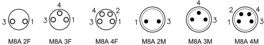
PIN ASSIGNMENT FRONT VIEW (前視圖)
