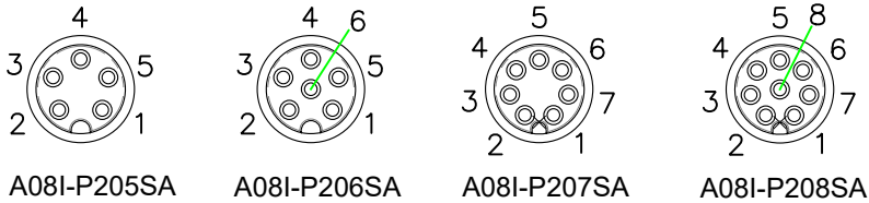
Pin Assignment Front View(前視圖)
