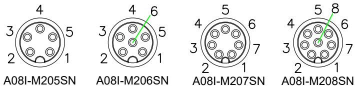
PIN ASSIGNMENT FRONT VIEW (前視圖) A1/B
