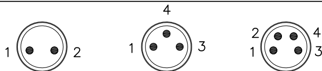
PIN ASSIGNMENT FRONT VIEW (前視圖)
