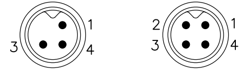
A05I-M103RM A05I-M104RM PIN ASSIGNMENT FRONT VIEW (前視圖)
