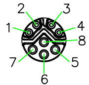
Pin Assignment Front View (前視圖)
