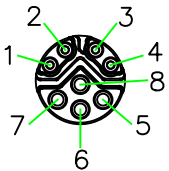
Pin Assignment Front View (前視圖)
