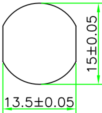
Recommended Panel Cut-Out
