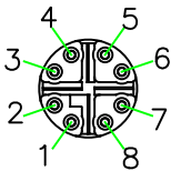
PIN ASSIGNMENT FRONT VIEW (前視圖)
