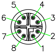
PIN ASSIGNMENT FRONT VIEW (前視圖)
