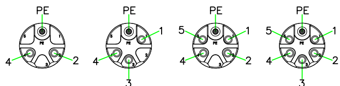
M12P-M603HSR M12P-M604HSR M12P-M605HSR M12P-M606HSR PIN ASSIGNMENT FRONT VIEW (前視圖)
