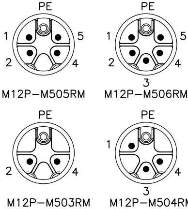
Pin Assignment Front View(前視圖)
