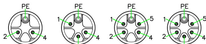
M12P-M503HSR M12P-M504HSR M12P-M505HSR M12P-M506HSR PIN ASSIGNMENT FRONT VIEW (前視圖)
