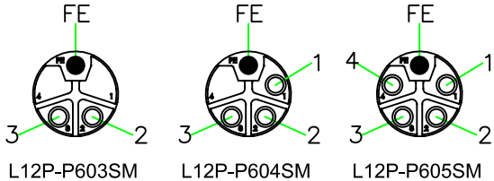
PIN ASSIGNMENT FRONT VIEW (前視圖)
