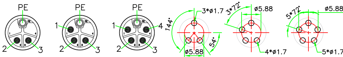
L12P-M503HPR L12P-M504HPR L12P-M505HPR L12P-M503HPR L12P-M504HPR L12P-M505HPR Pin Assignment Front View(前视图) PCB LAYOUT
