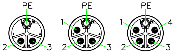
L12P-M503CSF L12P-M504CSF L12P-M505CSF PIN ASSIGNMENT FRONT VIEW (前視圖)
