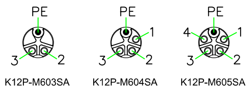
Pin Assignment Front View(前視圖)
