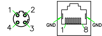
PIN ASSIGNMENT FRONT VIEW (前視圖)
