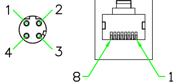
PIN ASSIGNMENT FRONT VIEW
