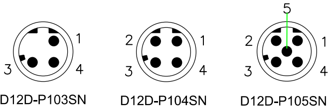
Pin Assignment Front View(前視圖)
