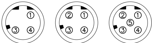
D12D-M103SAC D12D-M104SAC D12D-M105SAC PIN ASSIGNMENT FRONT VIEW (前視圖)
