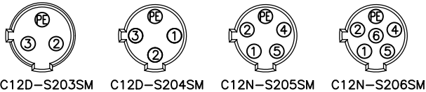
PIN ASSIGNMENT FRONT VIEW (前視圖)
