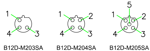
Pin Assignment Front View(前視圖)
