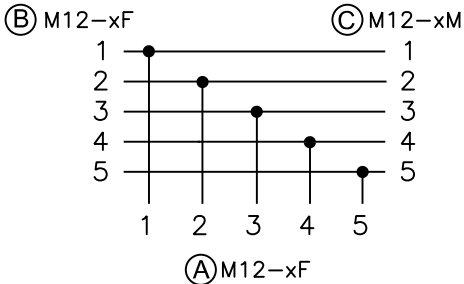
WIRING DIAGRAM
