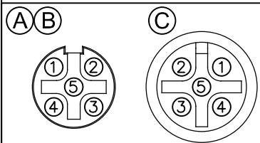
M12-xF M12-xM PIN ASSIGNMENT FRONT VIEW (前視圖)
