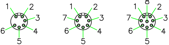
A12N-P206HPRR A12N-P207HPRR A12N-P208HPRR PIN ASSIGNMENT FRONT VIEW(前視圖)
