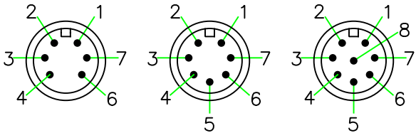
A12N-P106SA A12N-P107SA A12N-P108SA PIN ASSIGNMENT FRONT VIEW (前視圖)
