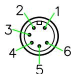
A12N-P106HPRR A12N-P107HPRR A12N-P108HPRR PIN ASSIGNMENT FRONT VIEW(前視圖)
