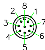
A12N-P106HPRR A12N-P107HPRR A12N-P108HPRR PIN ASSIGNMENT FRONT VIEW(前視圖)
