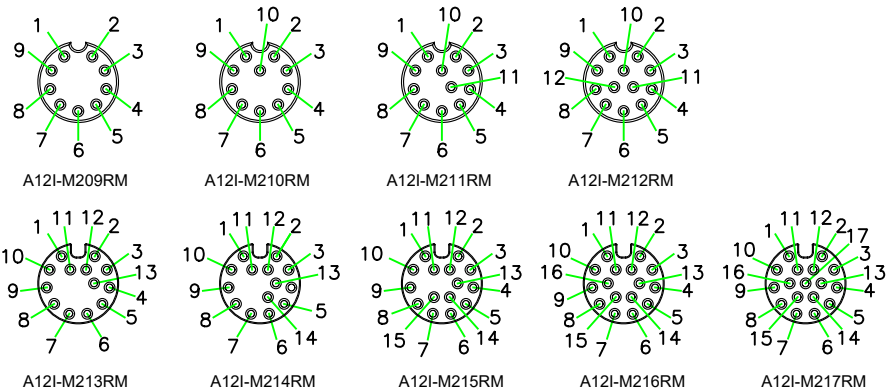
PIN ASSIGNMENT FRONT VIEW (前視圖)
