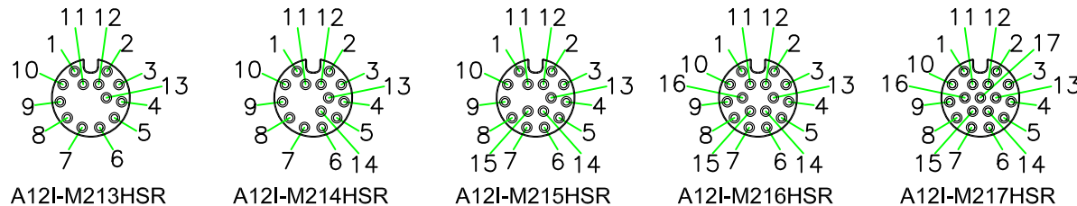
PIN ASSIGNMENT FRONT VIEW (前視圖)
