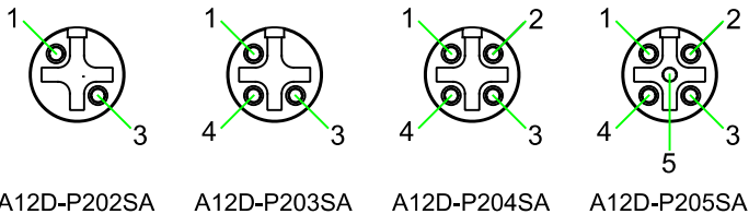
PIN ASSIGNMENT FRONT VIEW (前視圖)
