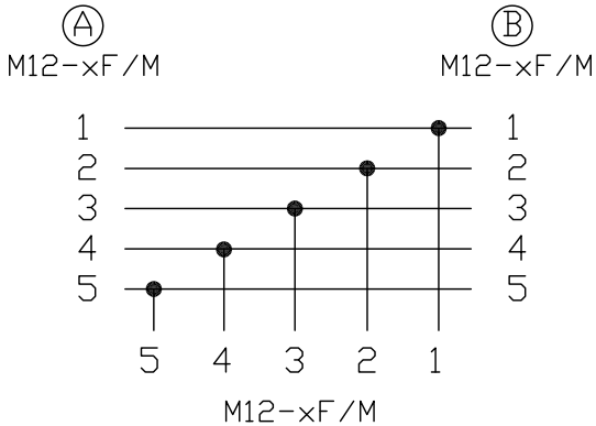
Wiring Diagram
