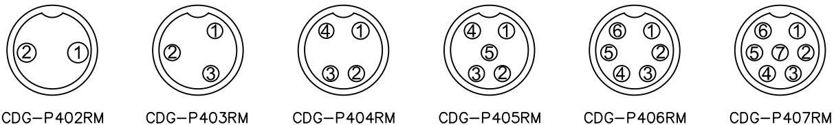
Pin Assignment Front View (前視圖)
