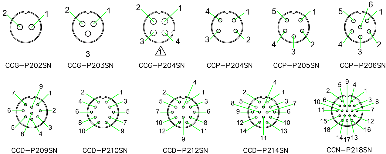
PIN ASSIGNMENT FRONT VIEW(前視圖)
