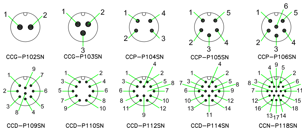
PIN ASSIGNMENT FRONT VIEW (前視圖)
