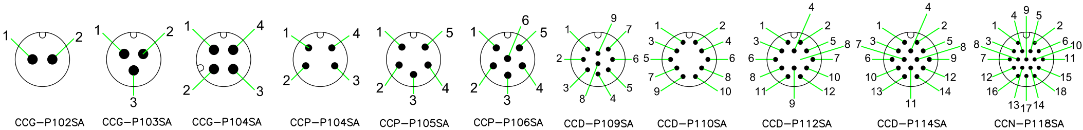
PIN ASSIGNMENT FRONT VIEW (前視圖)
