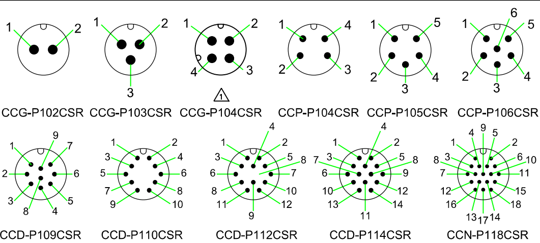
PIN ASSIGNMENT FRONT VIEW (前視圖)
