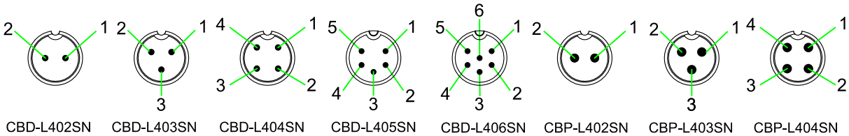
PIN ASSIGNMENT FRONT VIEW (前視圖)
