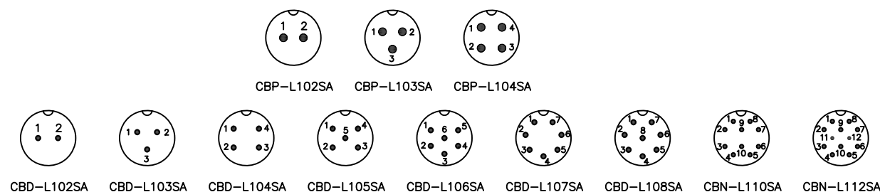
PIN ASSIGNMENT FRONT VIEW (前視圖) A
